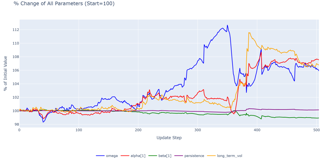
Figure 17: Parameter evolution over time
