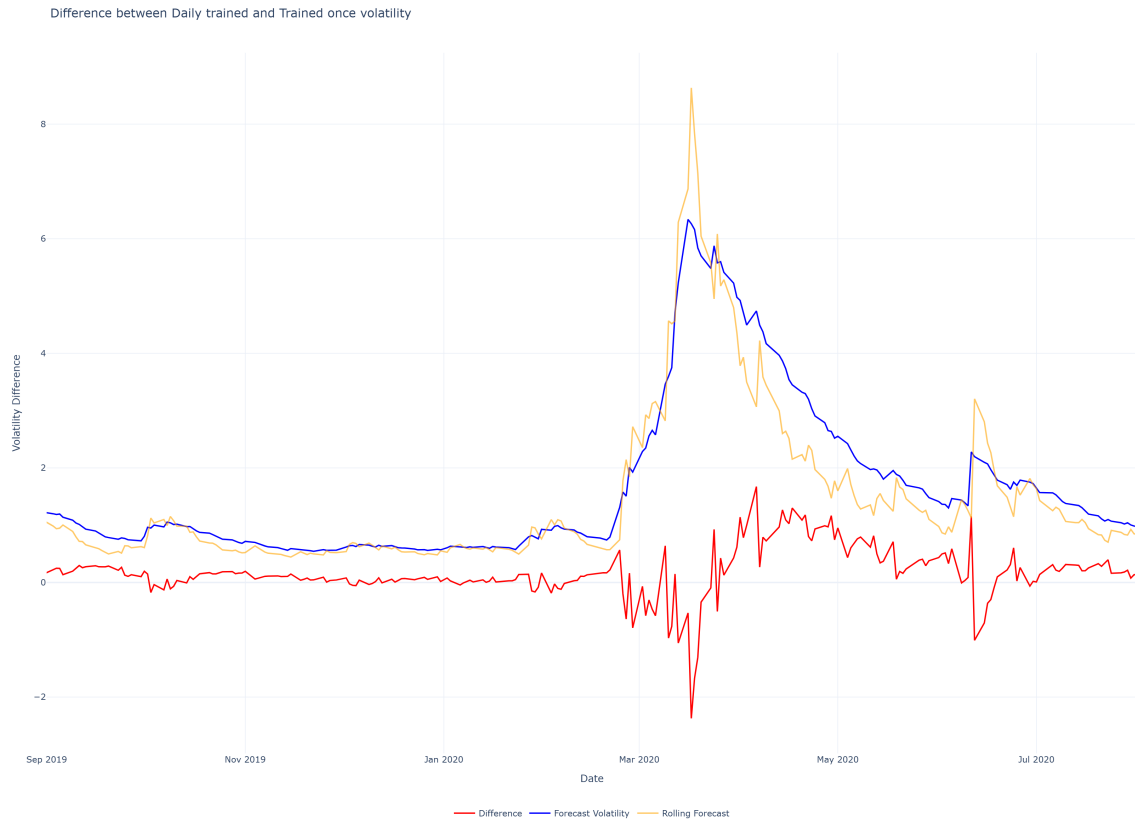
Figure 21: Zoomed Difference between Daily Trained and Trained Once model volatility
