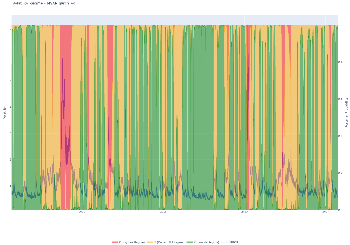
Figure 26: MSAR Regime Classifier GARCH
