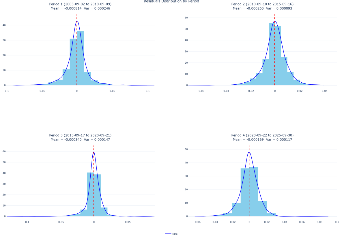
Figure 7: Distribution of shocks over the 4 periods
