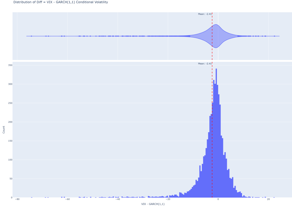
Figure 24: VIX - GARCH distribution
