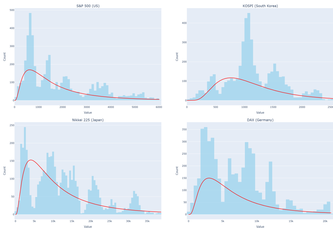
Figure 2: Log-Normal Prices Distribution
