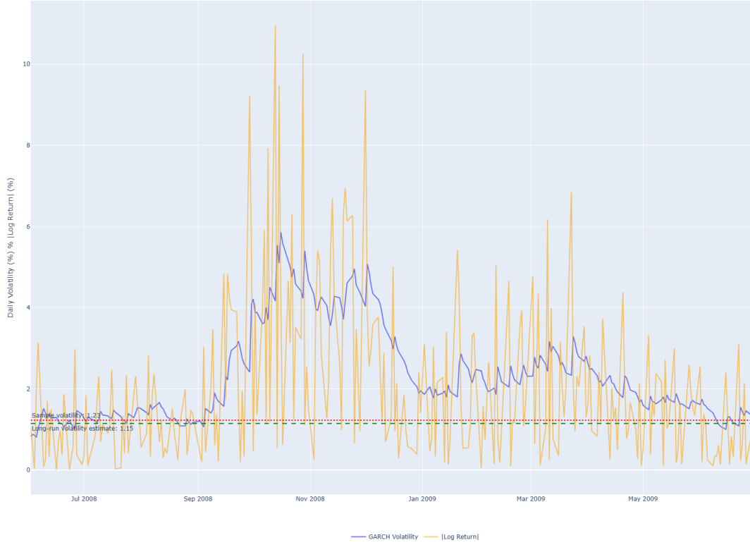
Figure 9: Absolute returns and Volatility (Zoomed in)
