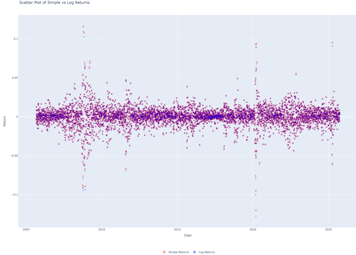
Figure 4: Simple vs Log Returns Scatter Plot
