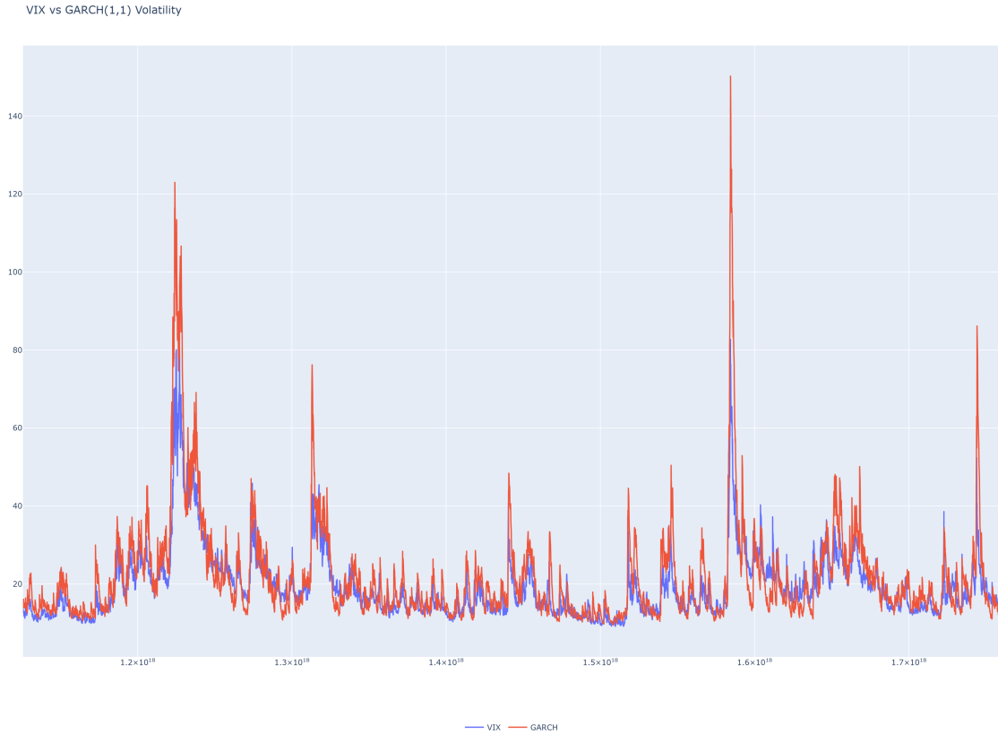
Figure 23: Vix vs GARCH volatility
