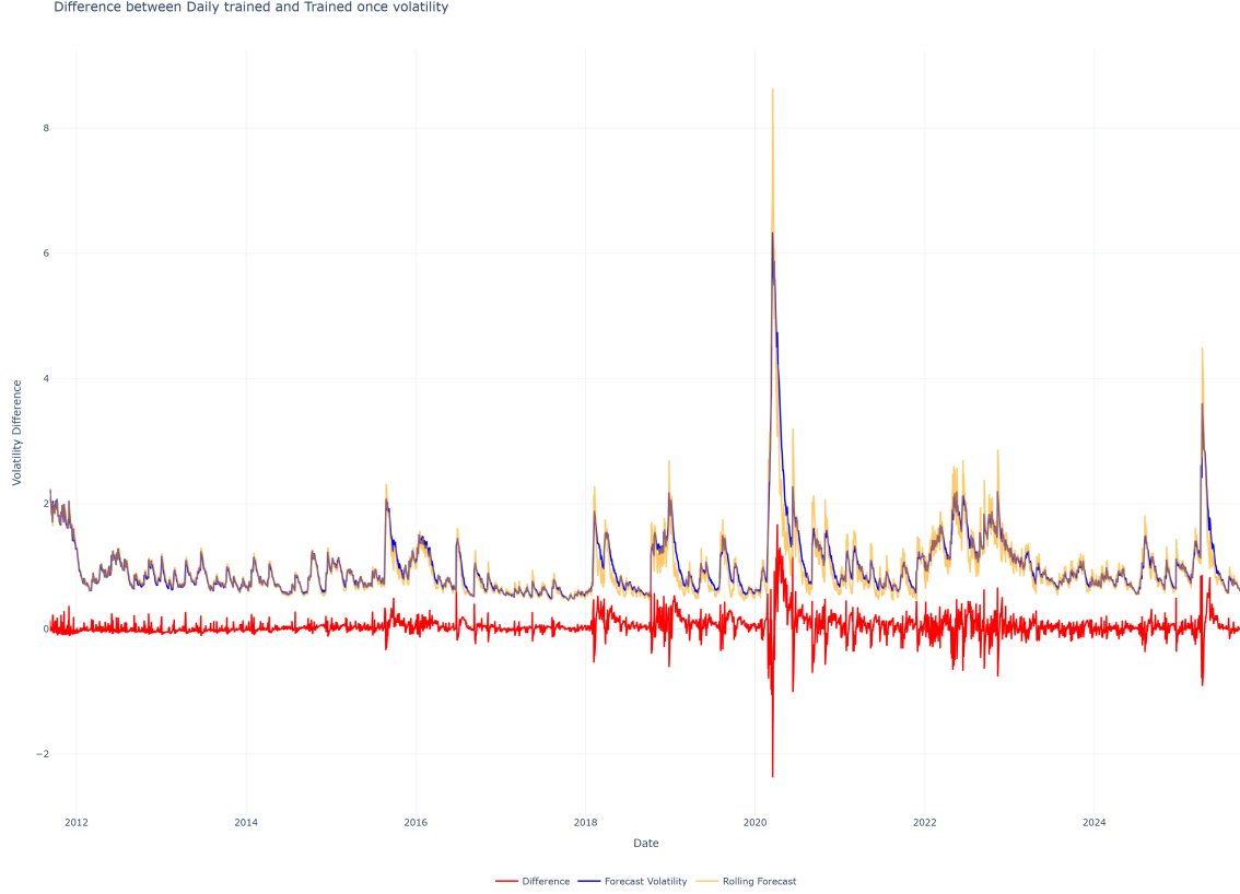
Figure 20: Difference between Daily Trained and Trained Once model volatility
