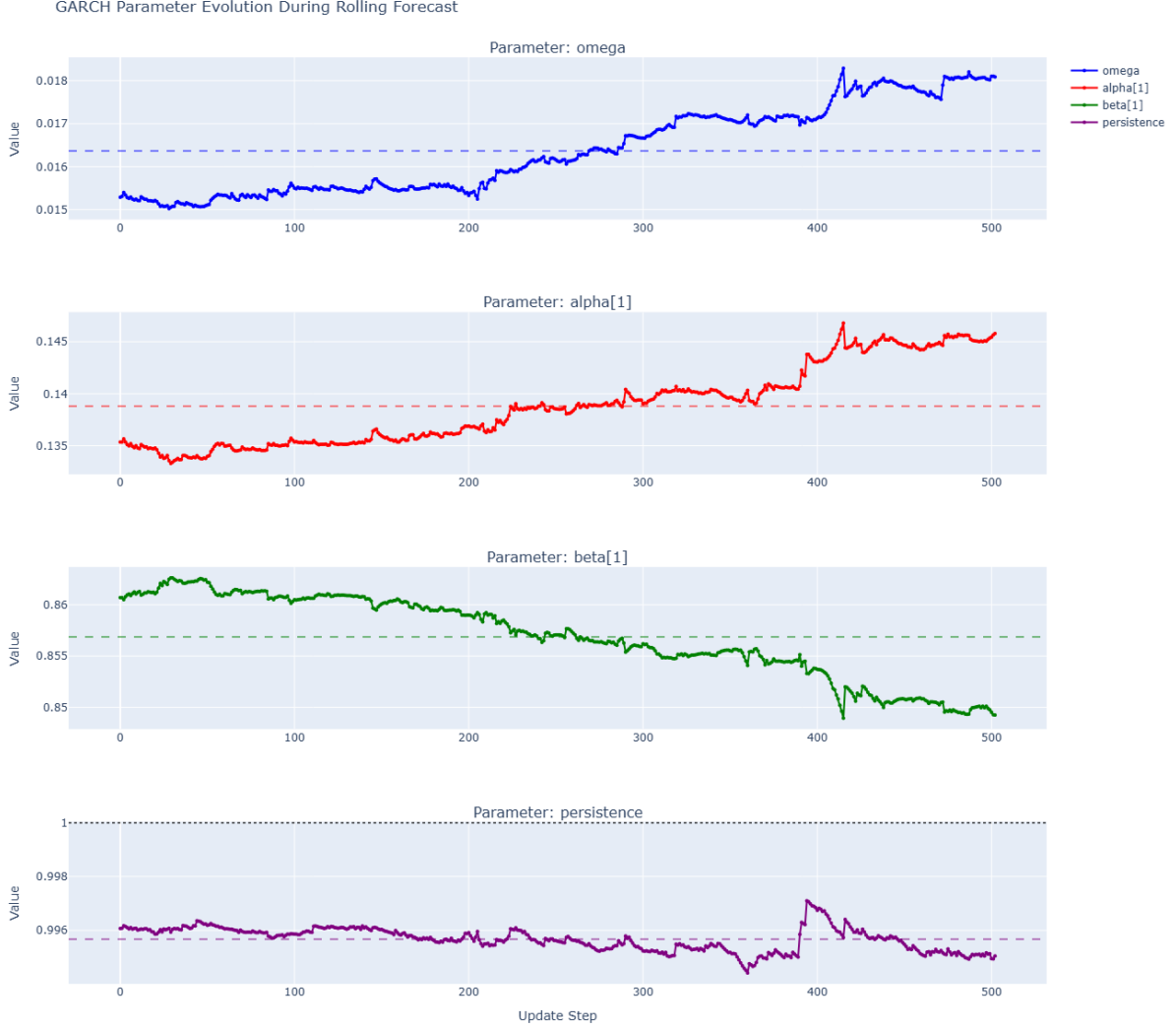
Figure 16: Parameter evolution over time
