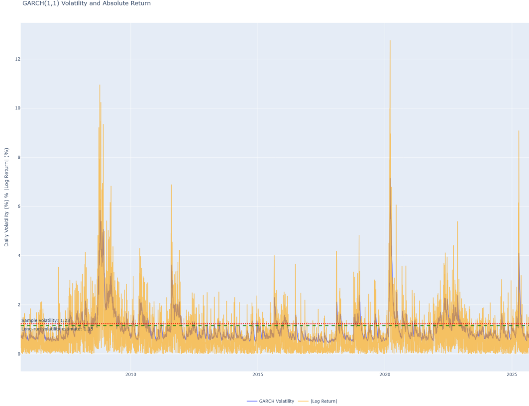
Figure 8: Volatility and Absolute Returns
