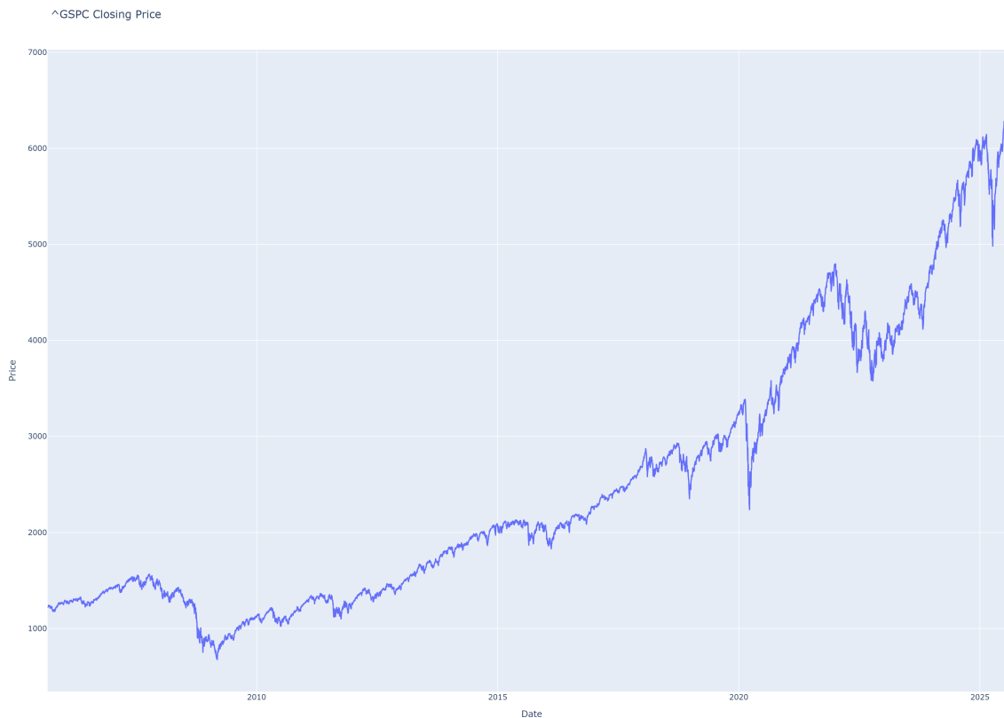
Figure 1: SP500 Closing Price History
