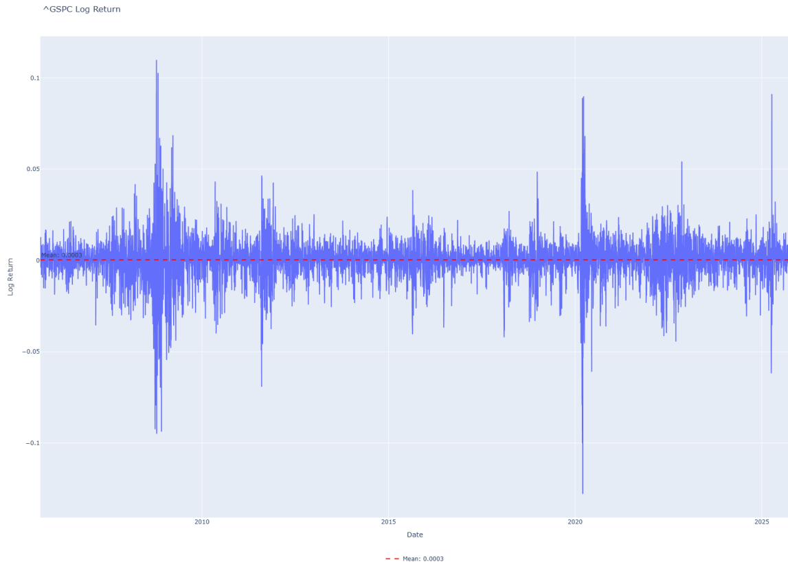
Figure 3: Log Returns over time
