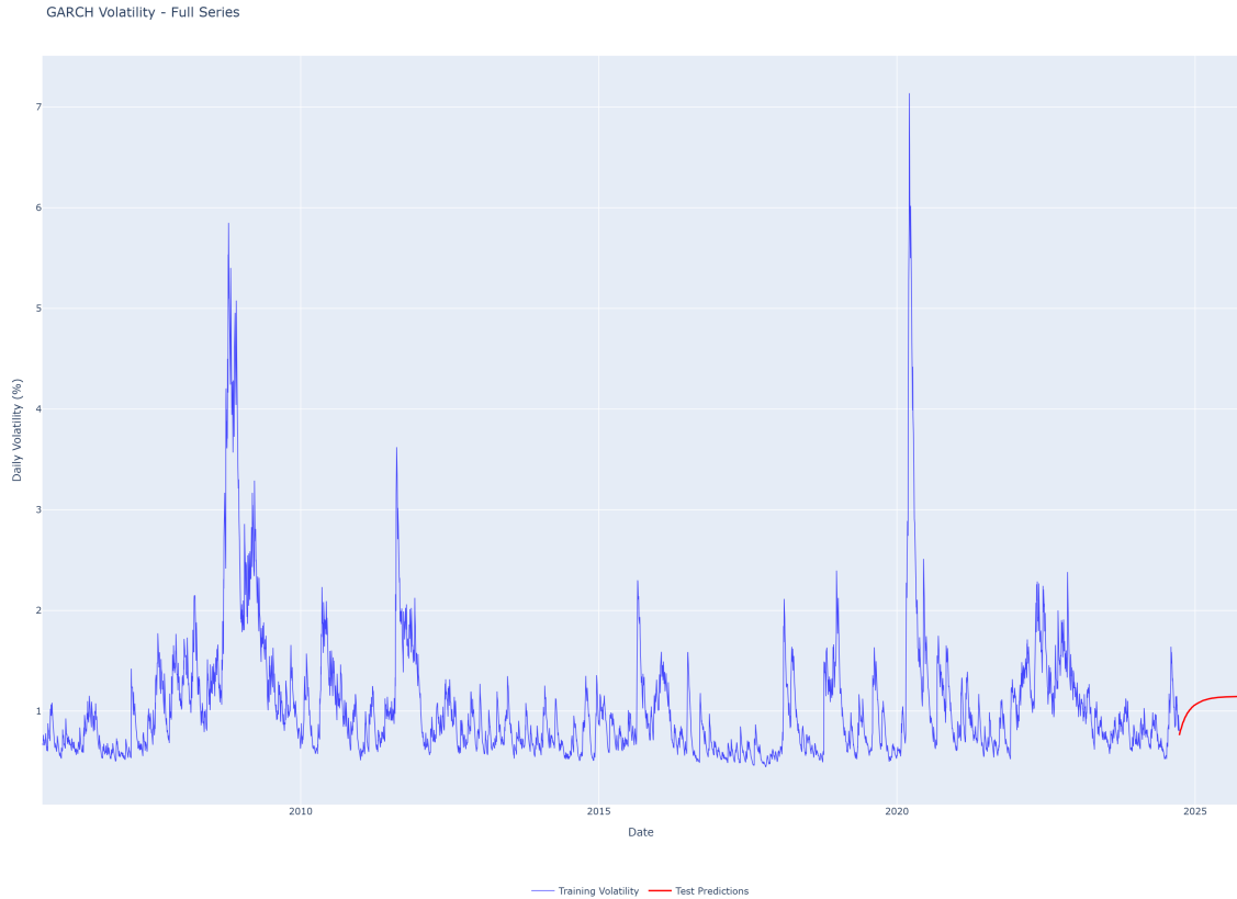
Figure 13: Trained Model Conditional Vol. and 1y Predicted Vol.
