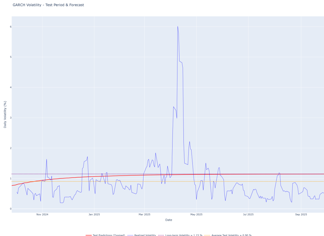
Figure 14: Test period: Prediction vs Realized volatility
