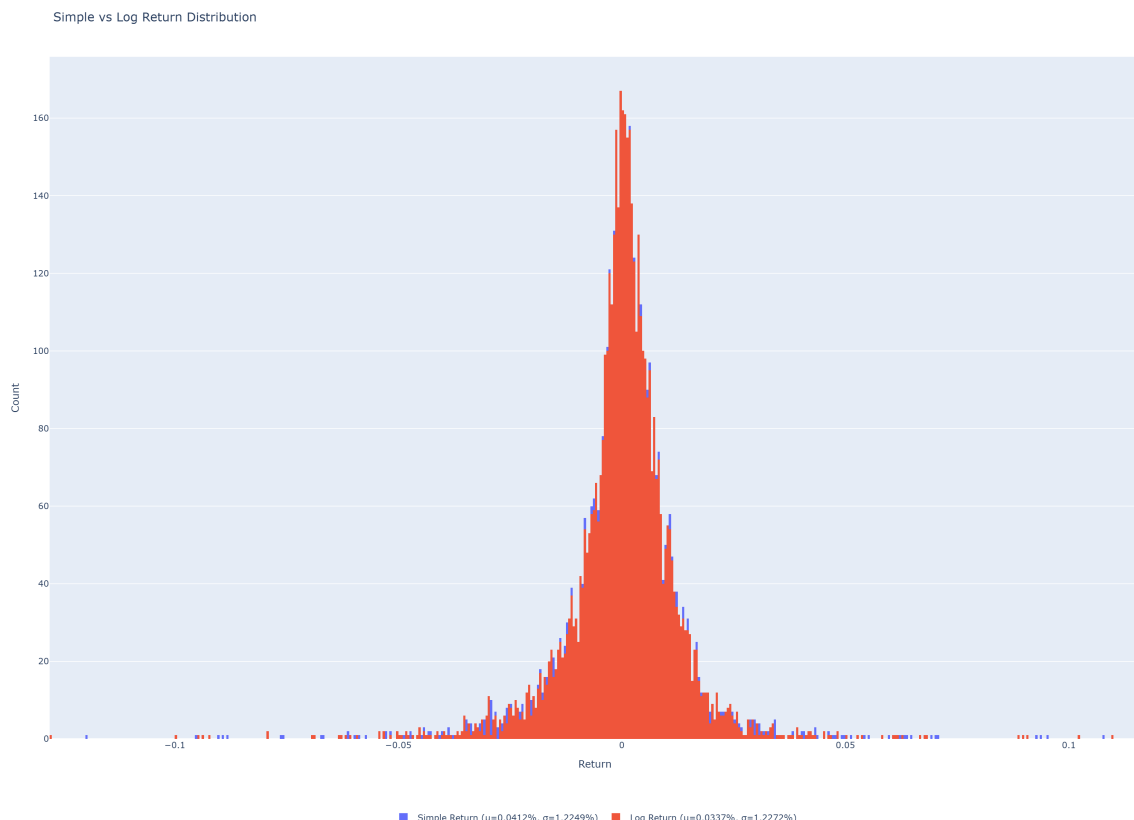
Figure 5: Distribution of Simple vs Log Returns
