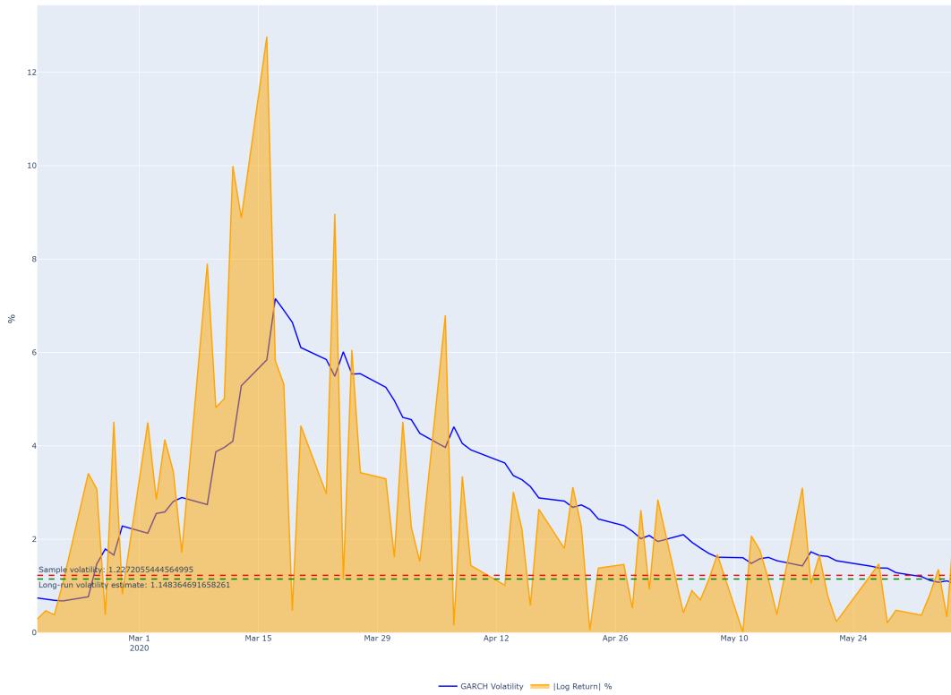
Figure 11: Persistence of volatility
