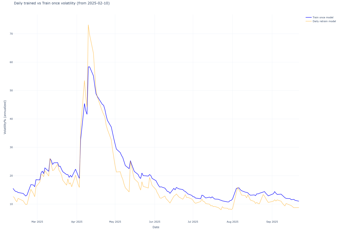
Figure 19: Zoomed Daily Trained model vs Trained Once model
