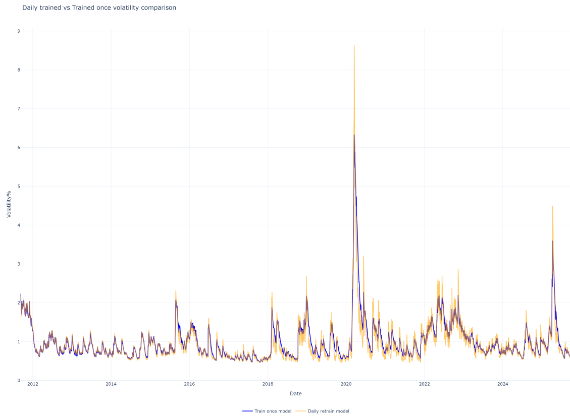
Figure 18: Daily trained vs Trained Once conditional volatilities
